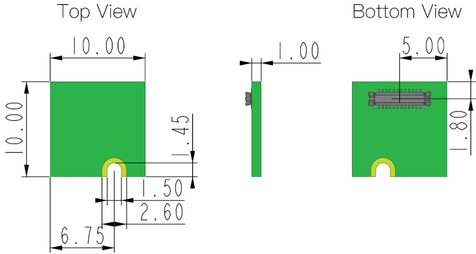
Figure 5: RAK12003 WisBlock Infrared Temperature Sensor Mechanic Drawing
