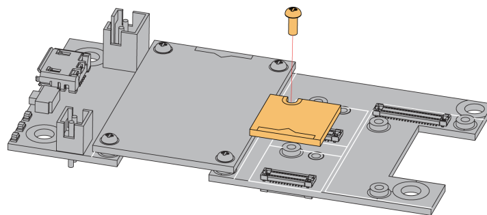
Figure 2: RAK12003 WisBlock Infrared Temperature Sensor Mounting
