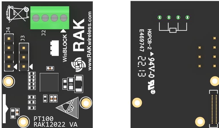
Figure 1: RAK12022 WisBlock PT100 Module
