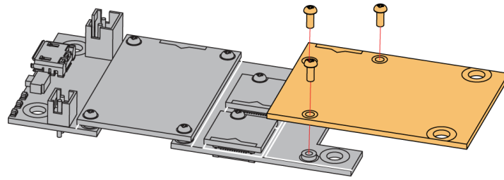
Figure 2: RAK12022 WisBlock PT100 Module Mounting
