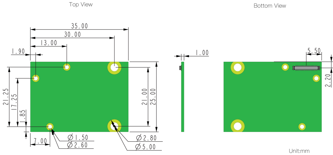
Figure 4: RAK12022 WisBlock PT100 Module Mechanical Drawing
