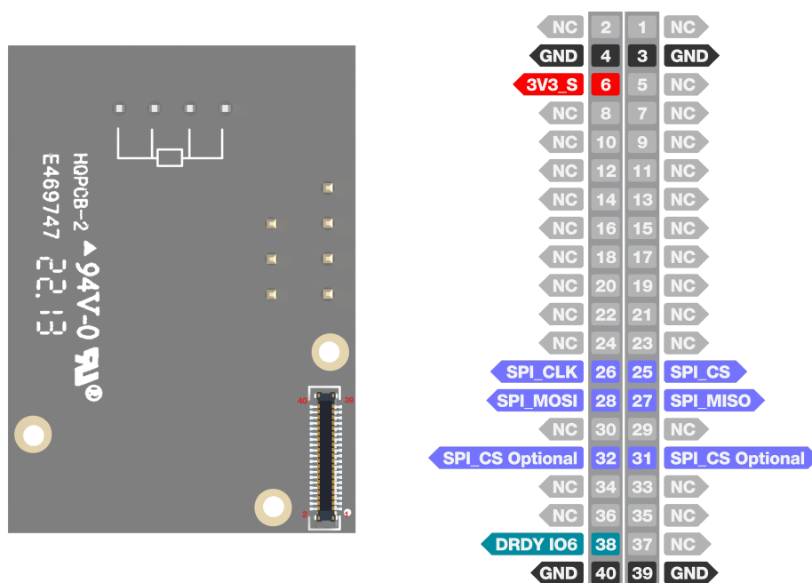
Figure 3: RAK12022 WisBlock PT100 Module Pinout
