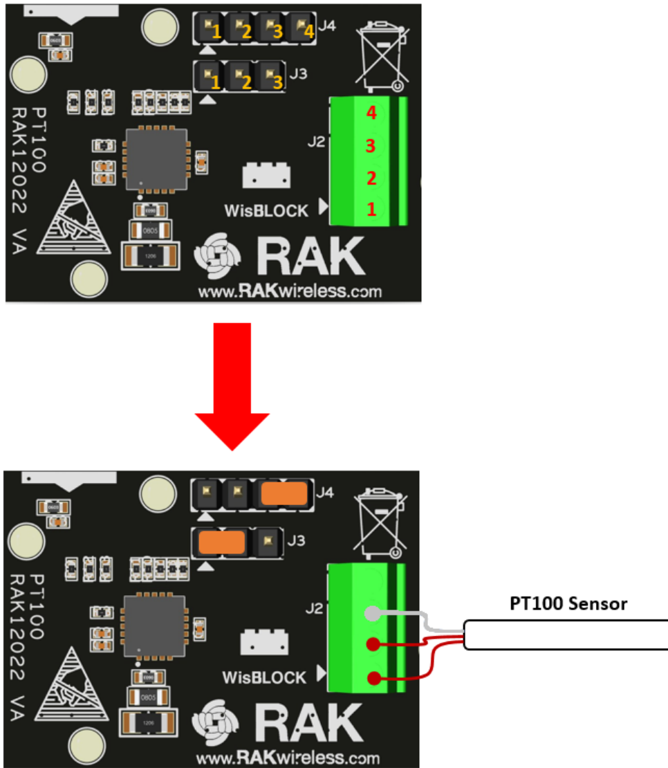
Figure 8: RAK12022 WisBlock PT100 Module 3-Wire Connection
