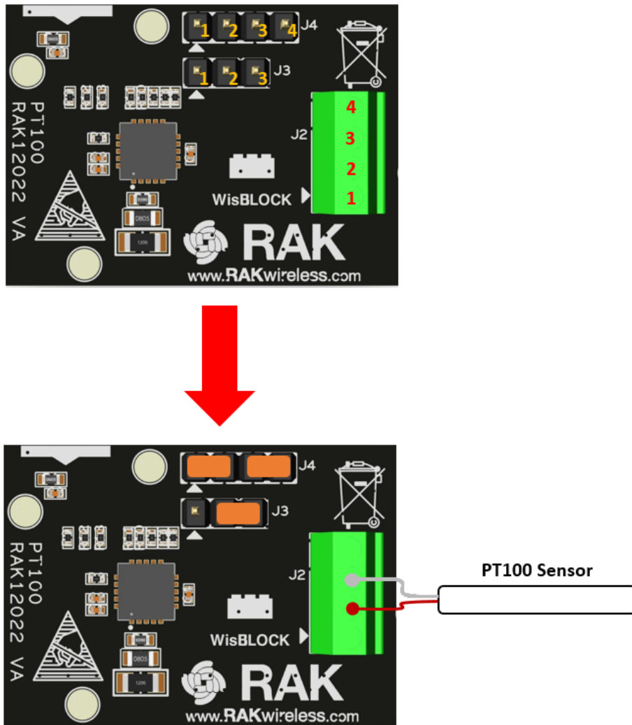
Figure 7: RAK12022 WisBlock PT100 Module 2-Wire Connection
