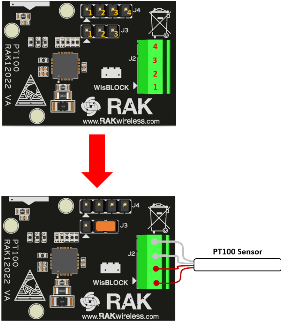
Figure 9: RAK12022 WisBlock PT100 Module 4-Wire Connection
